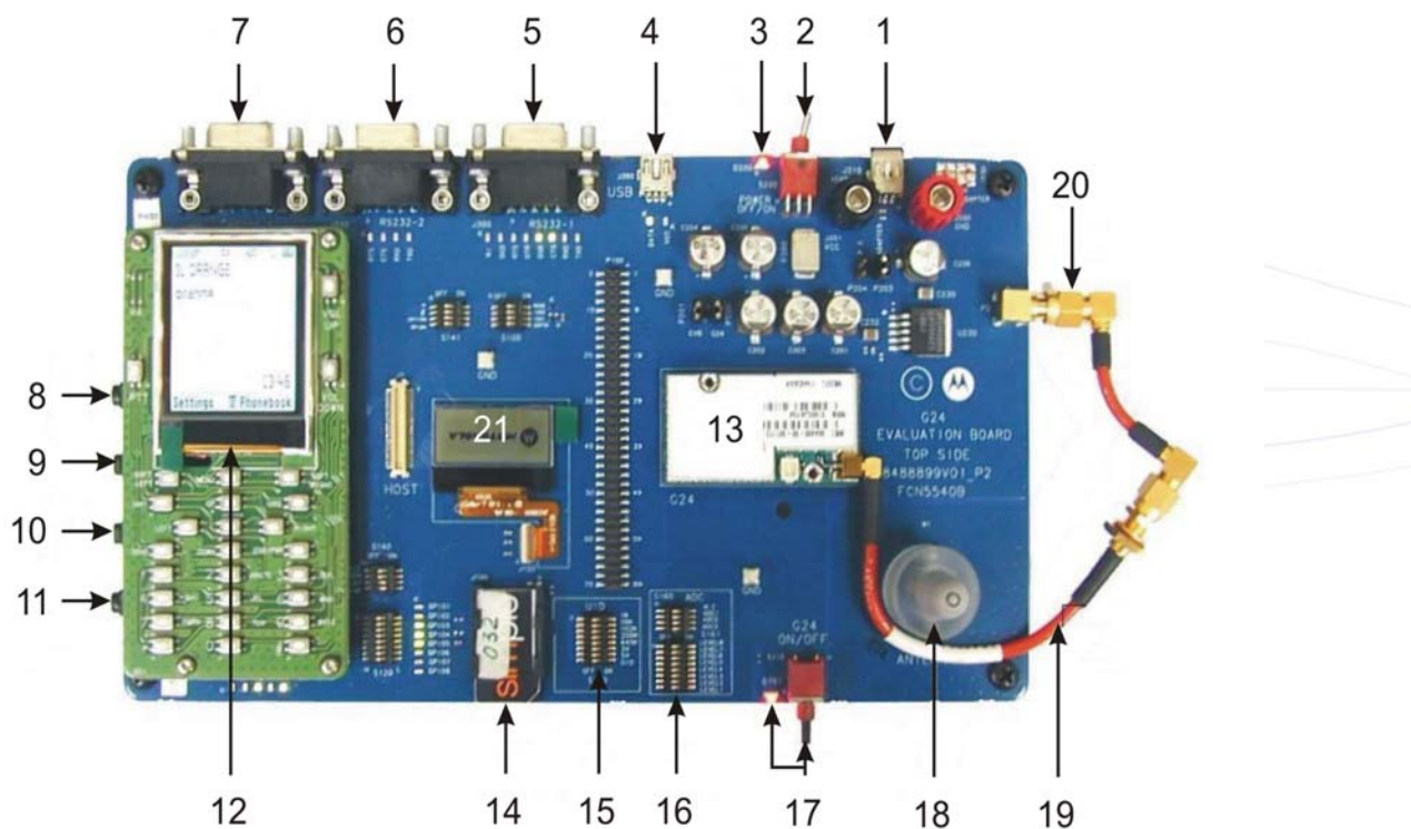
Figure 2-1: Evaluation Board - Major Components
