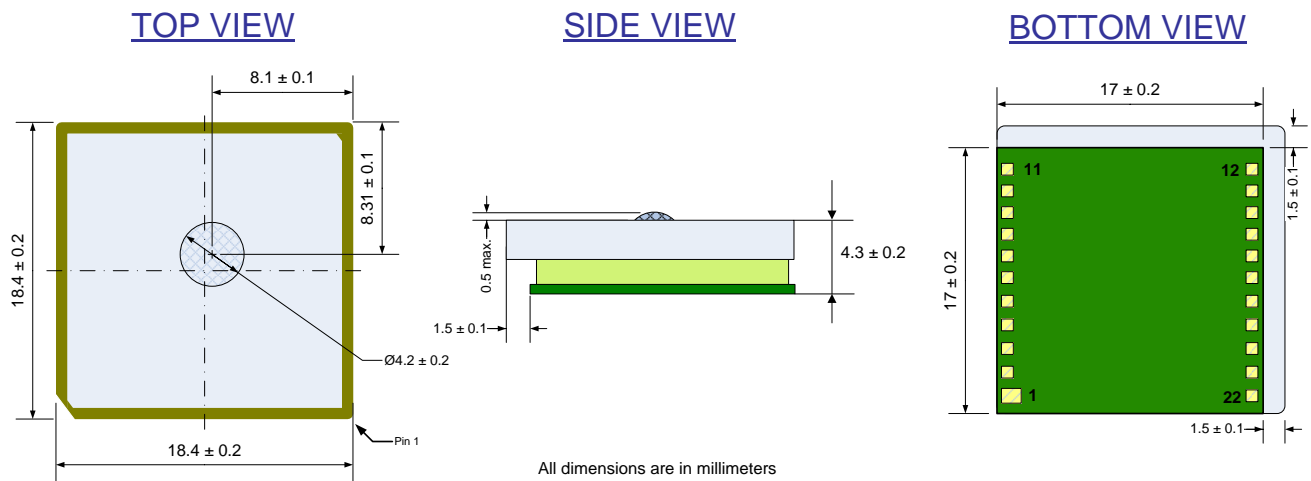
Figure 9-3: ORG-1318 mechanical drawing
