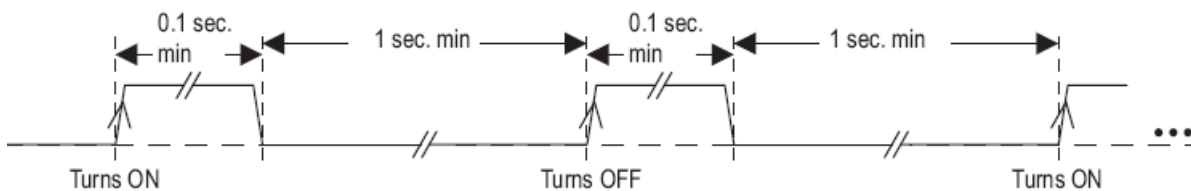
Figure 6-1: ON_OFF timing
