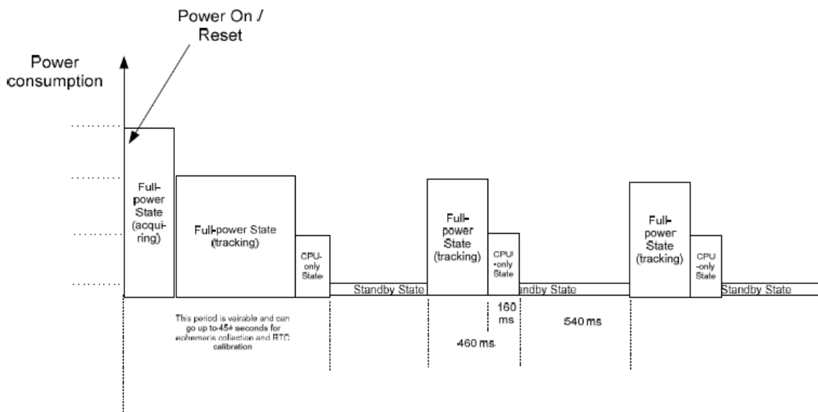
Figure 5-1: ATP timing
