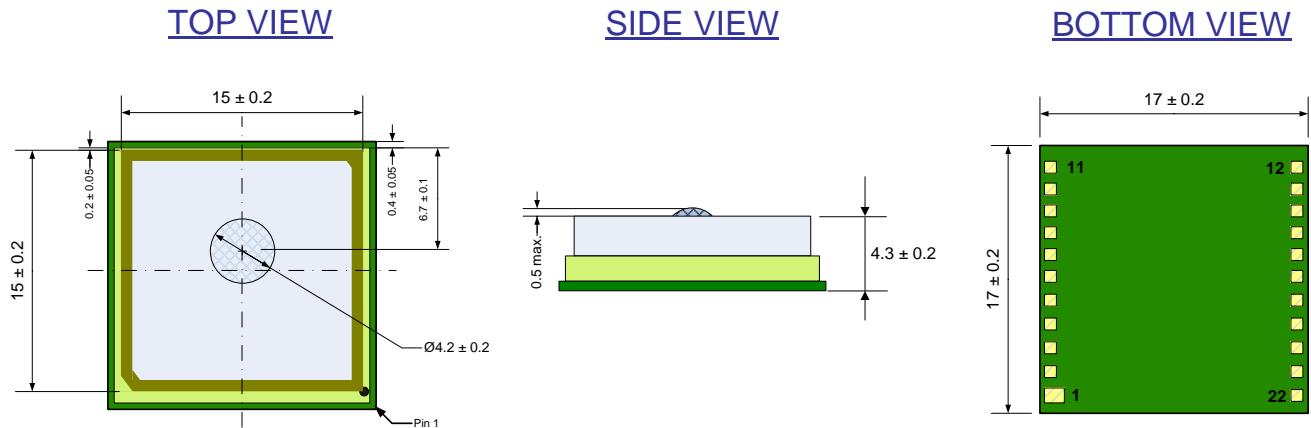
Figure 9-2: ORG-1315 mechanical drawing
