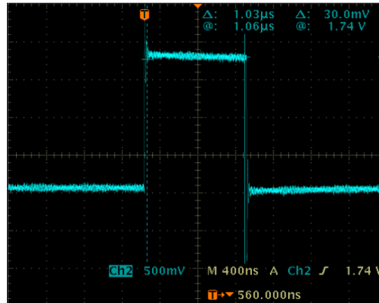
Figure 6-3: 1PPS
