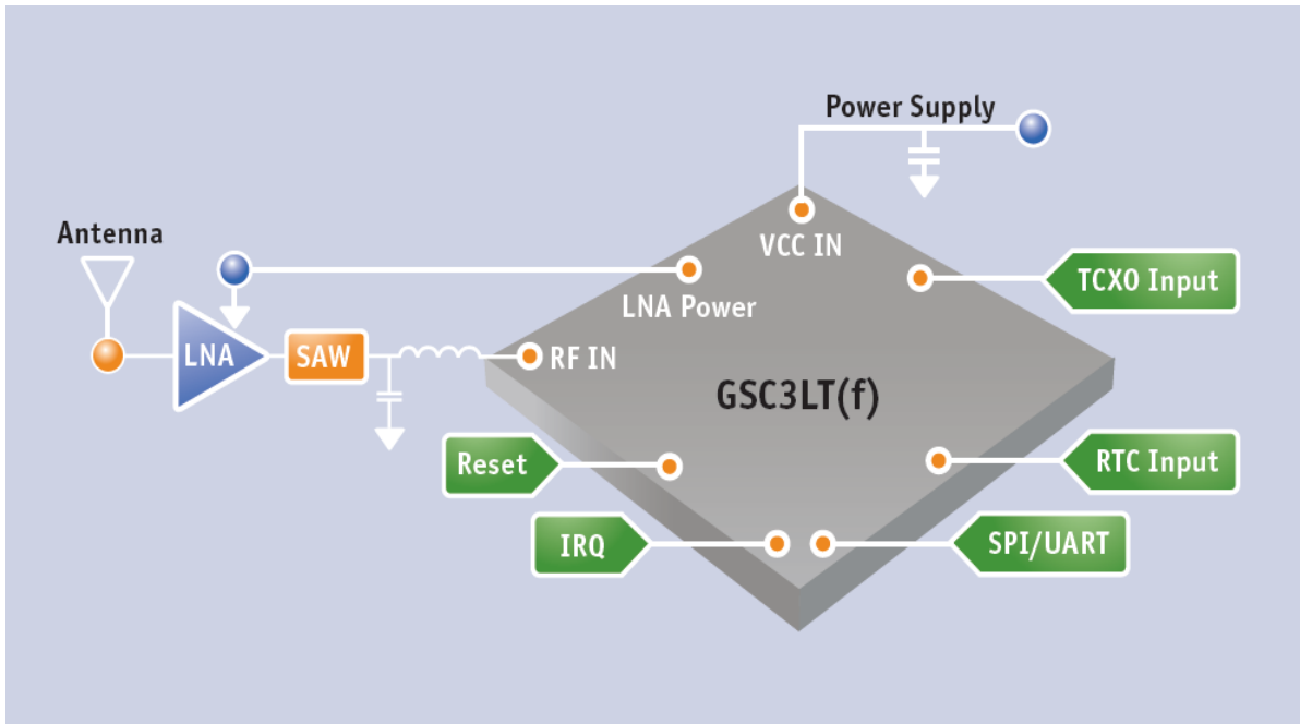
Figure 2-1: ORG-13XX architecture
