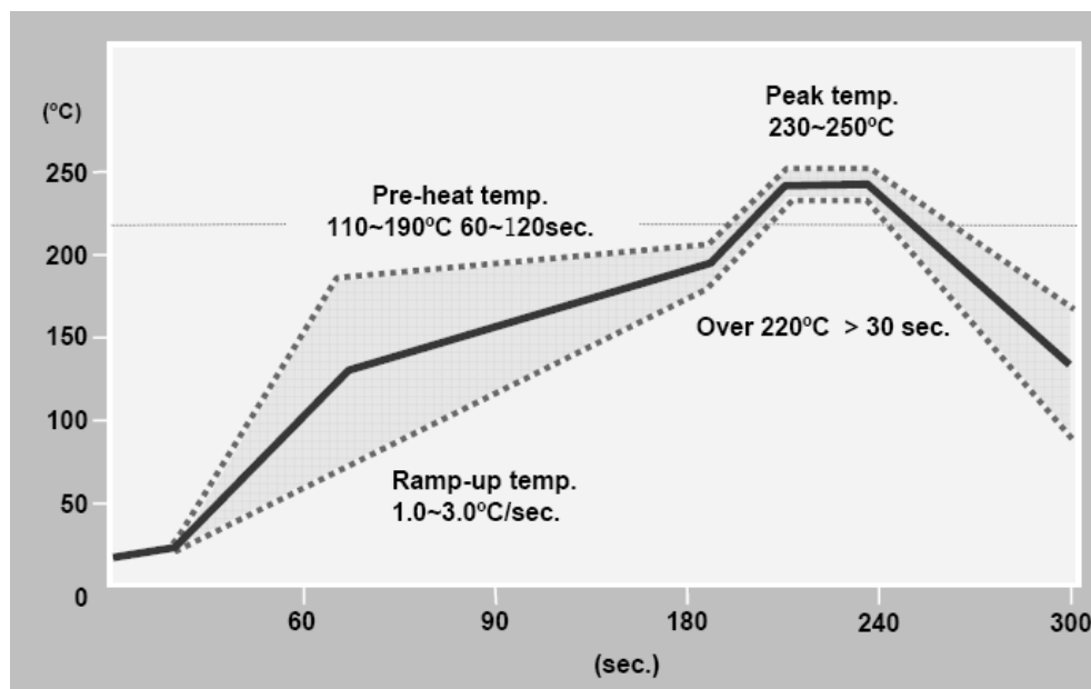
Figure 8-4: Recommended soldering profile
