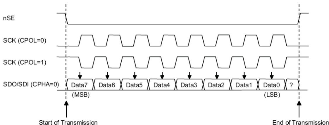
Figure 6-2: SPI timing
