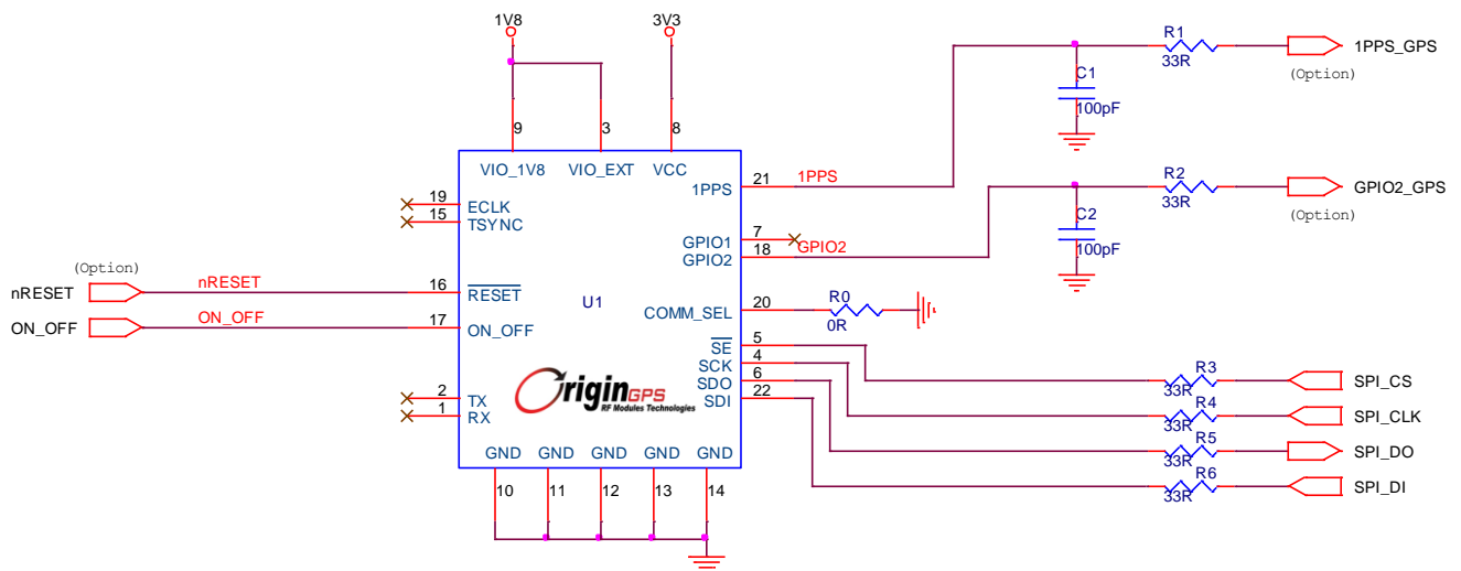
Figure 6-7: SPI communication circuit
