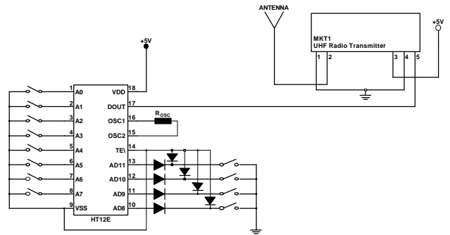
Figure 3: MK Transmitter Application Circuit
