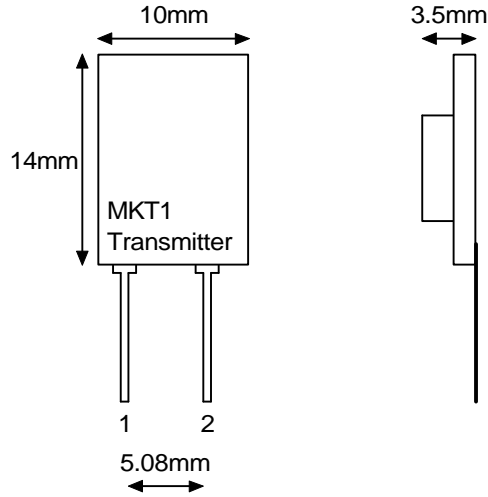
Figure 4: MKT1 Transmitter
