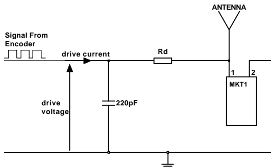
Figure 2: Drive Circuit Required For MKT1 Transmitter Module
