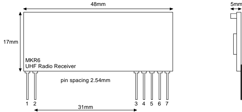
Figure 4: RS-MKR6 Receiver
