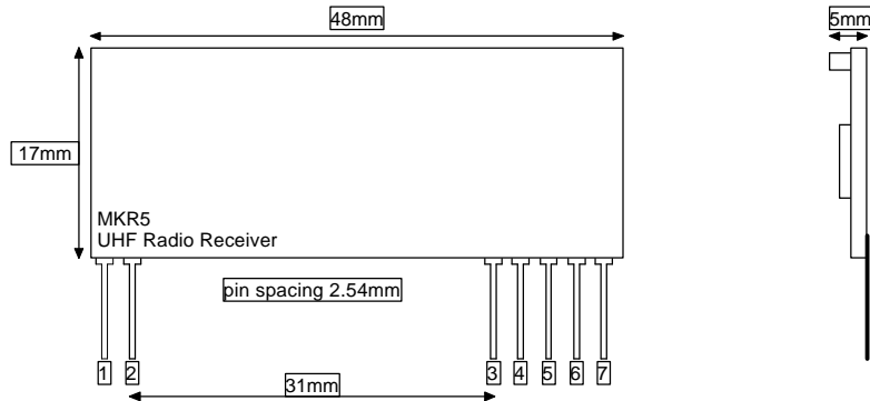
Figure 4: MKR5 Receiver
