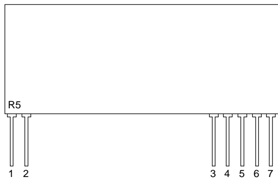
Figure 1: MKR5 Receiver
