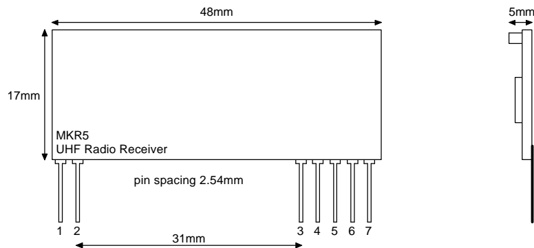
Figure 4: RS-MKR5A Receiver
