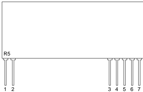
Figure 1: RS-MKR5A Receiver
