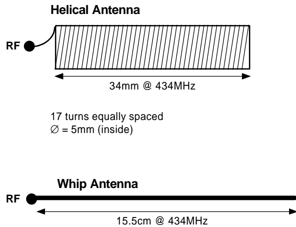
Figure 3: Antenna configurations to be used with the RS-MK modules
