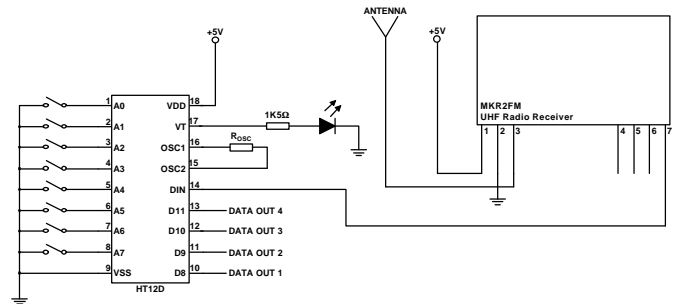
Figure 4: RS-MKR2FM Receiver Application Circuit
