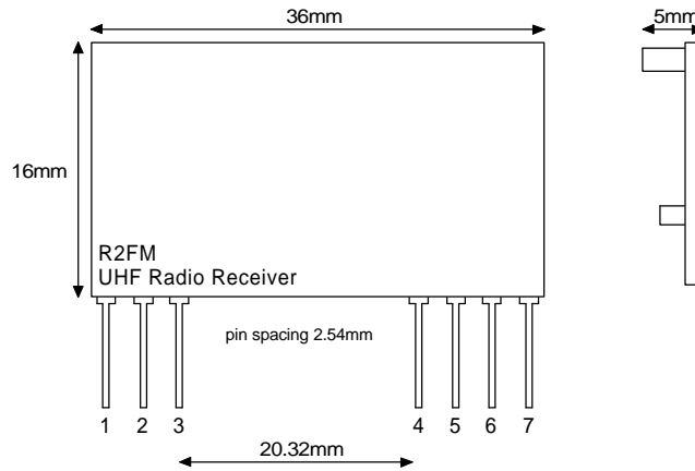
Figure 5: RS-MKR2FM Receiver
