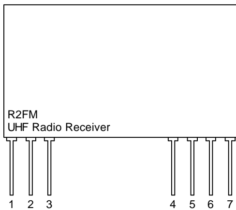
Figure 1: RS-MKR2FM Receiver
