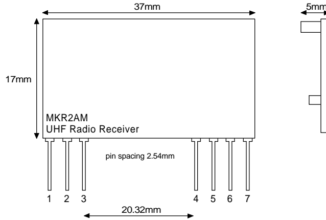
Figure 5: RS-MKR2AM Receiver
