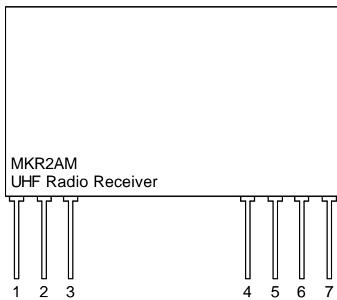
Figure 1: RS-MKR2AM Receiver
