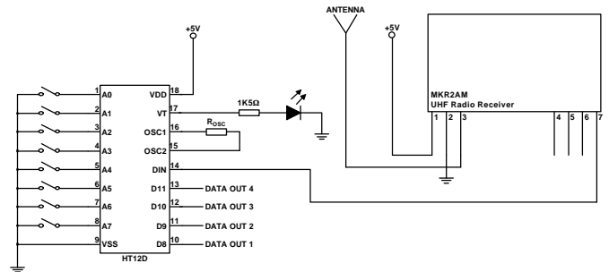
Figure 4: RS-MKR2AM Receiver Application Circuit
